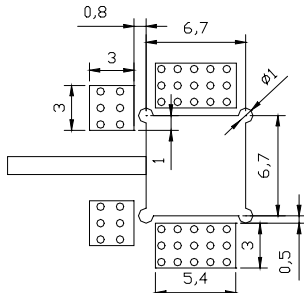
PCB Land Pattern for Mounting VEREND
